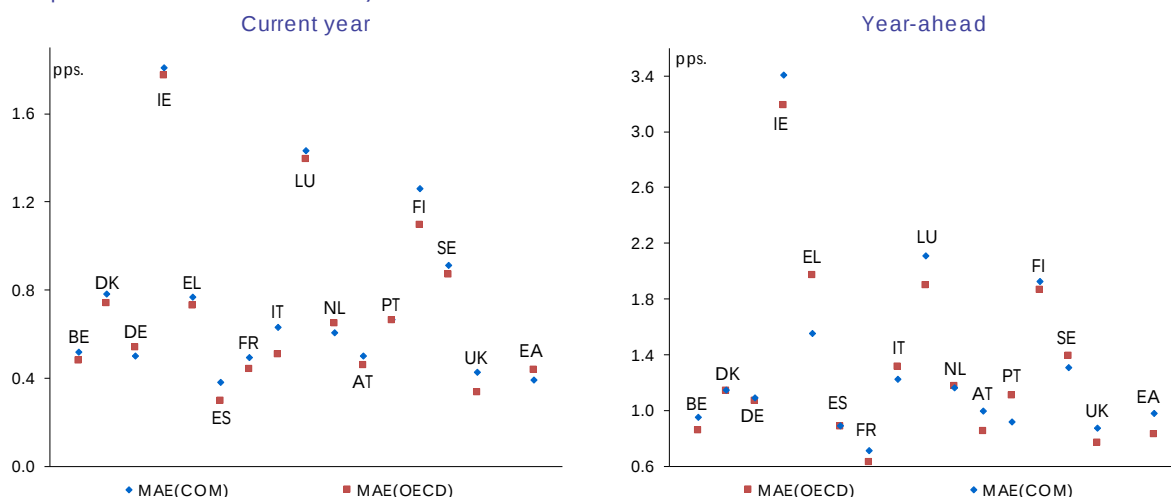
Graph 6.1.: Mean absolute error, 2000-2017
