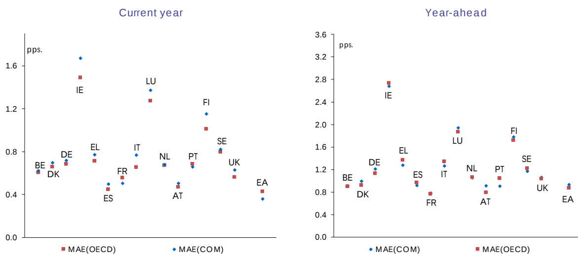
Graph A.3: Mean absolute error, EC and OECD forecasts, 1969-2017
