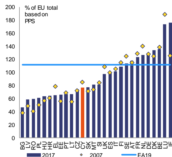
Graph 4.4.1: Labour productivity
